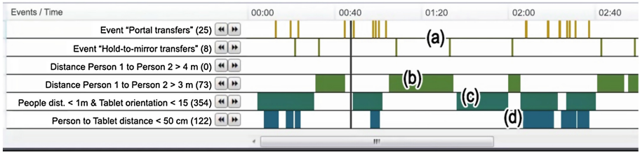
Fig. 3. Analysis generated through queries to the EXCITE tool.
