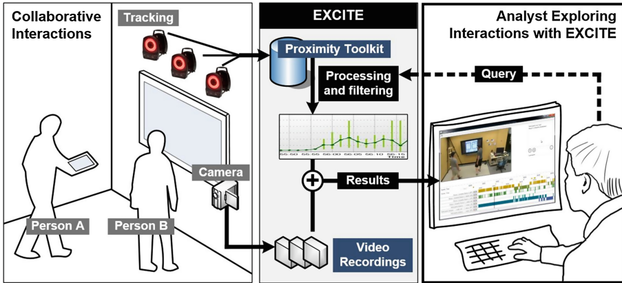
Fig. 1. EXCITE overview: Capturing video, tracking data, and application events (center) in collaborative environments (left), and providing querying interface and visualizations to allow analysis of group interactions (right).
