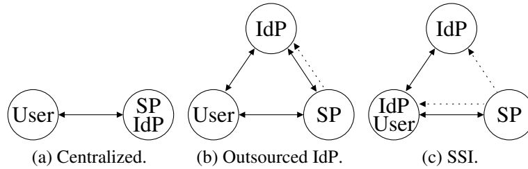
Figure 2 – IAM models.
