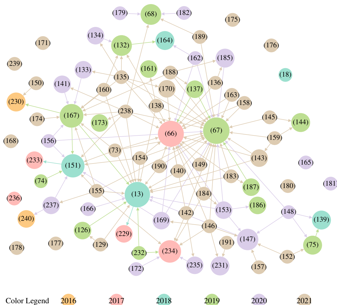
Figure 14 – Co-reference network.
