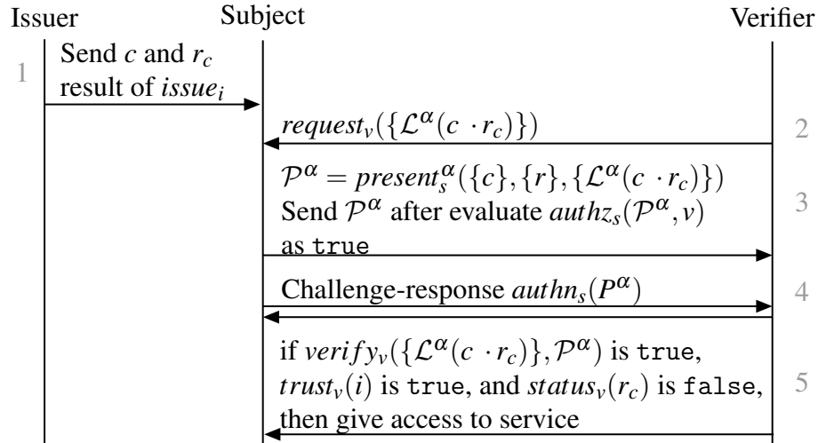
Figure 20 – An instance of the OffOldPM high-level protocol.
